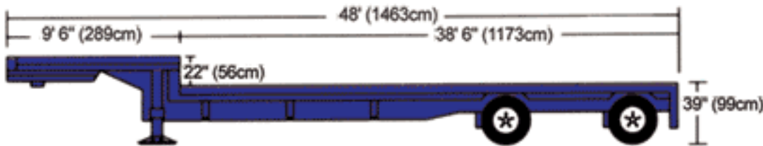
Drop Deck 2 Axle Spread
