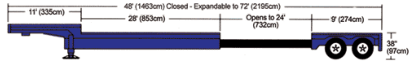
Expandable Drop Deck 2 or 3 Axle
