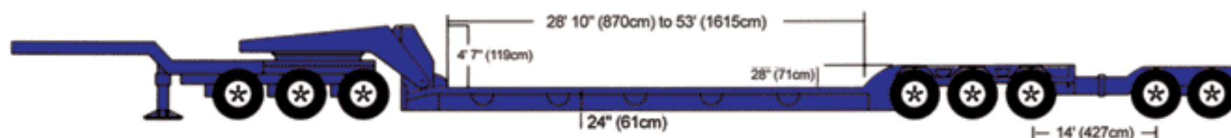
Multiple Axle High Tonnage Flatbed
