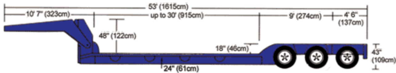
Multiple Axle High Tonnage Double Drop (Floor Deck)
