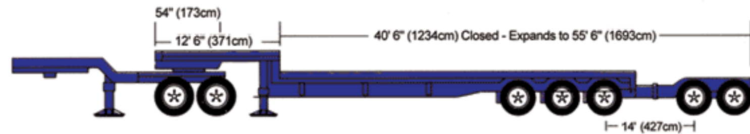
Multiple Axle High Tonnage Spread Axle Single Drop Expandable
