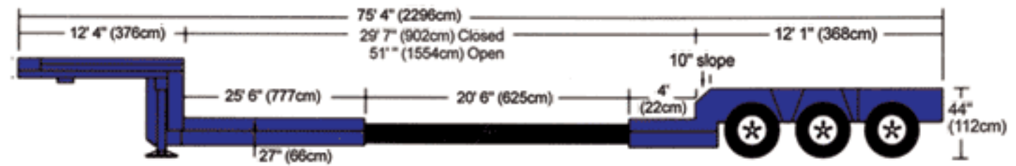
Expandable Double Drop Deck 3 Axle
