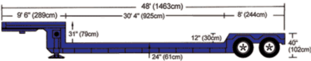
RGN Double Drop Deck 2 Axle
