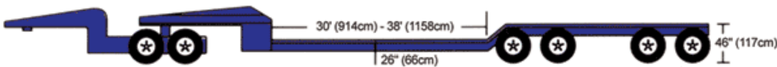
Multiple Axle High Tonnage Double Drop
