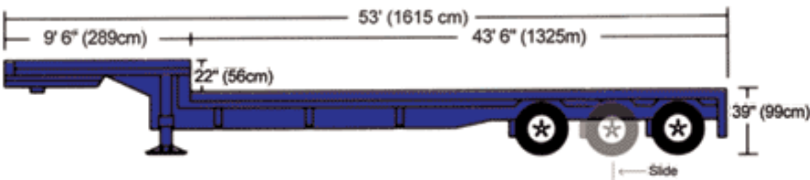
53' Drop Deck with Sliding Rear Axle
