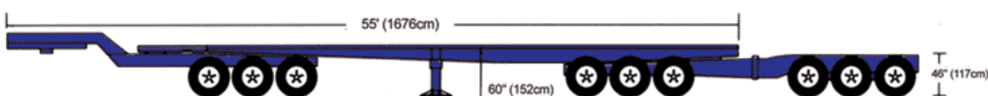
Multiple Axle High Tonnage Flatbed
